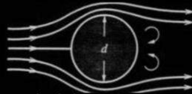
Blunt body
