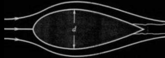
Streamlined body
